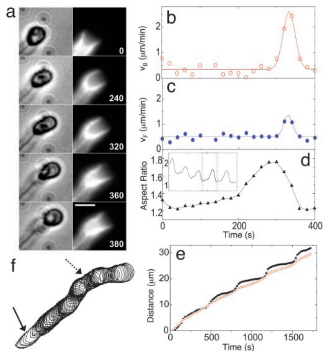
Fig. 3. Dynamics of the elongation and release of a vesicle from the actin gel. (a) Time sequence of phase-contrast (Left) and fluorescence (Right) images of a vesicle going through a slow-elongation and rapid-release phase. Phase-contrast images show the vesicle and a trailing comet tail. Fluorescence images show the intensity of rhodamine-actin in gray scale. The actin cup elongates from an initial shallow shape and creeps around the vesicle, becoming shallow again as the vesicle appears to be released suddenly from the cup and becomes spherical. The time elapsed in seconds is shown on the bottom right corner of the fluorescence images. (Scale bar, 3 \mu\text{m} .) (b and c) Instantaneous velocity of the back ( V_B ) and front ( V_F ) of the moving vesicle as a function of time. Time-lapse images acquired at intervals of 20 sec were used to quantify the velocity and shapes. The solid lines are a guide to the eye. (d) Aspect ratio of vesicle shape as a function of time. Aspect ratio is defined as the maximum length divided by the maximum width perpendicular to the length. The highest velocity occurs just after the vesicle reaches its maximum length. (Inset) Aspect ratio of a vesicle that repeats the elongation-relaxation cycle several times. The vertical dotted lines indicate the part of the time series that is shown in greater detail in d. (e) The distance traveled by the front (open circles) and back (filled circles) of a stepping vesicle, as a function of time. (f) Overlay of vesicle contours from phase-contrast images at successive time steps (20-sec intervals) of motion, showing oscillations in velocity. In regions where the contours are further apart (solid arrow), the trailing edge of the vesicle moves rapidly; regions of densely packed contour lines (dashed arrow) depict slower forward motion during vesicle elongation.
